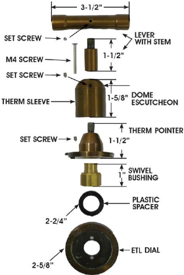
THERM PLATE
